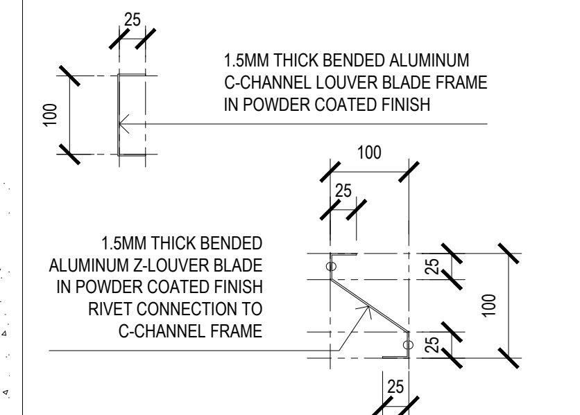
ALUMINUM LOUVER CHANNEL & BLADE PROFILE SCALE 1:05
