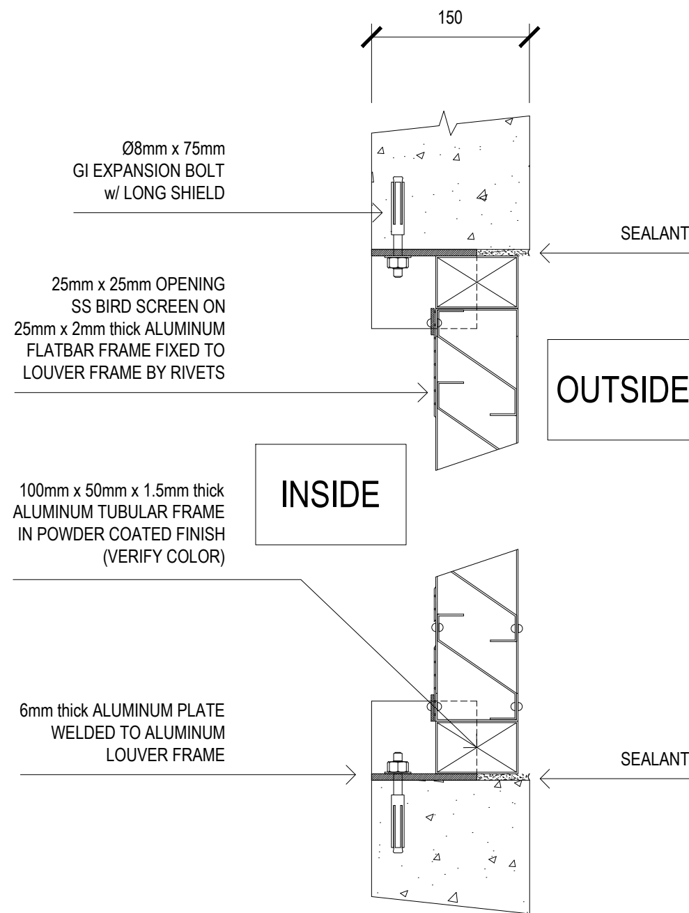
ALUMINUM LOUVER LOUVER DETAILED SECTION TYP. SCALE NTS
