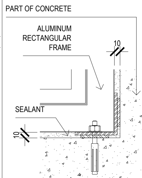
ALUMINUM LOUVER BLOW-UP 02 SCALE 1:04
